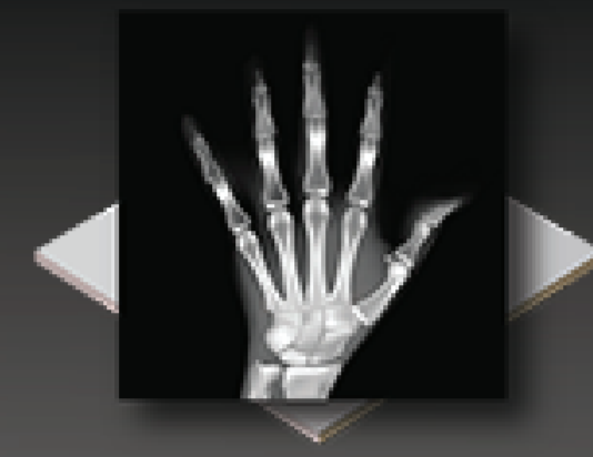
X-ray / Rayon X
