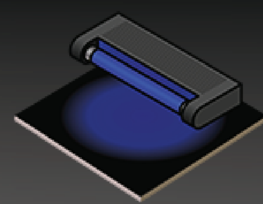
Ultraviolet / Rayon ultraviolet
