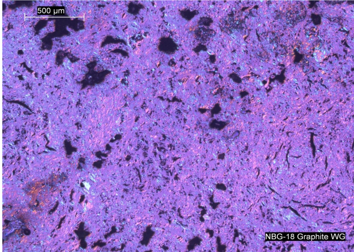
Grade NBG-18 graphite (with-grain) microstructure (viewed under polarized light)
