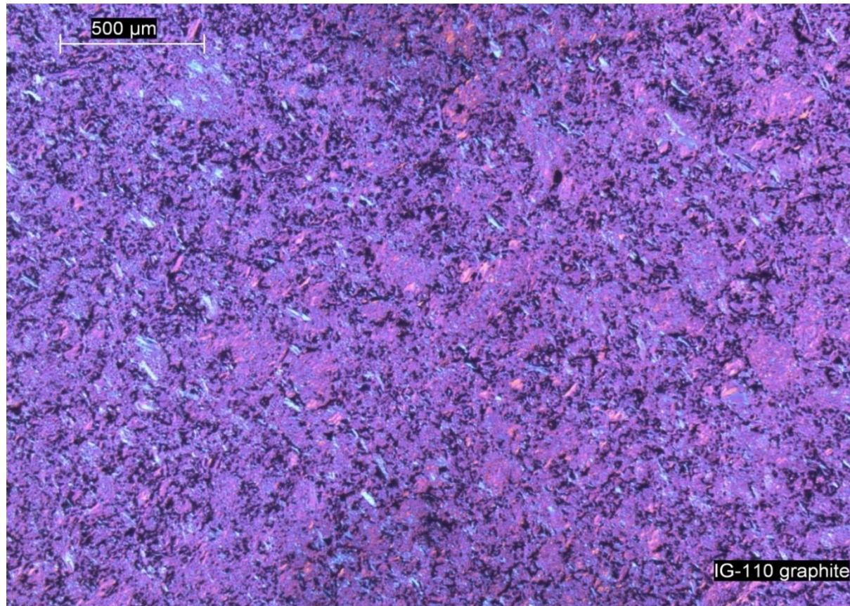
Grade IG-110 graphite microstructure (viewed under polarized light)
