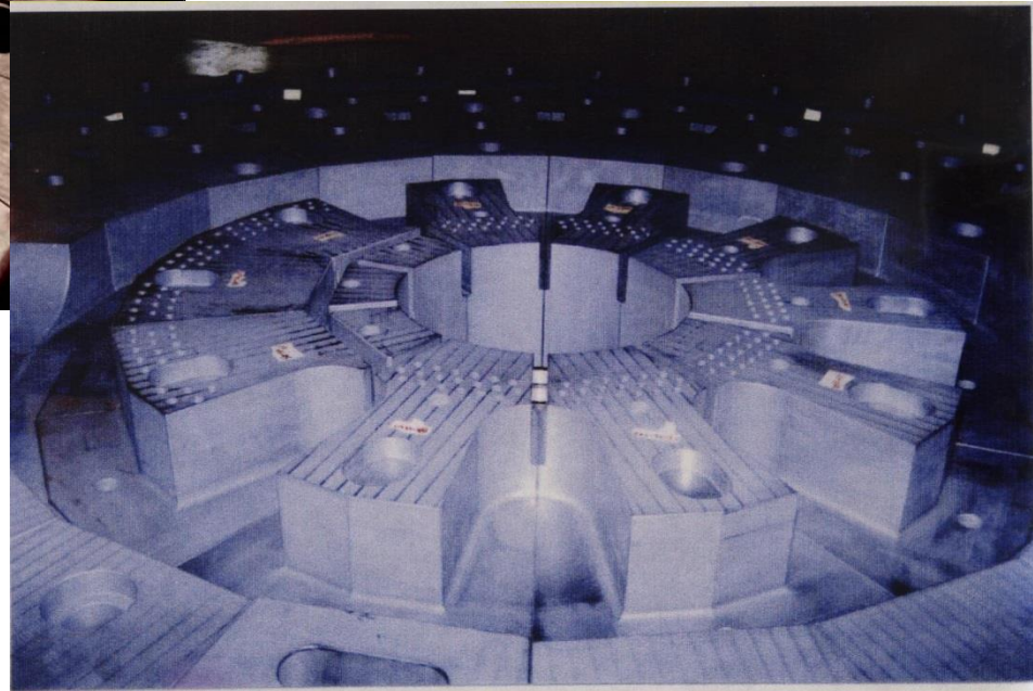
Core bottom of the HTR-10 showing the fuel pebble collection area
