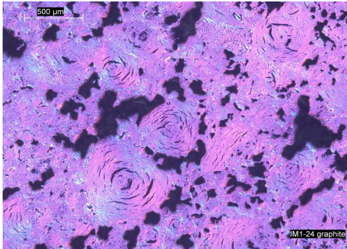
Grade IM1-24 graphite microstructure (viewed under polarized light)
