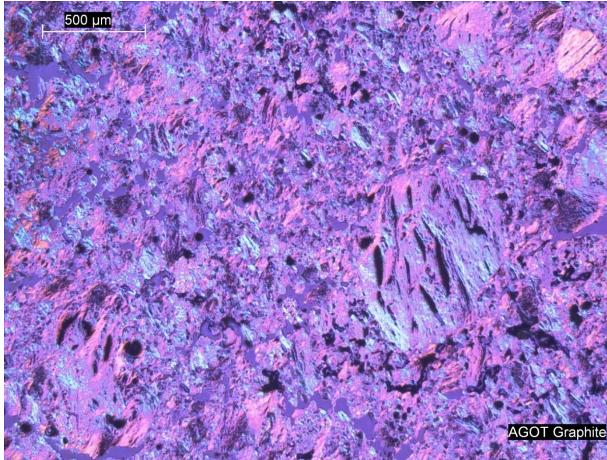
Grade AGOT graphite microstructure (viewed under polarized light)
