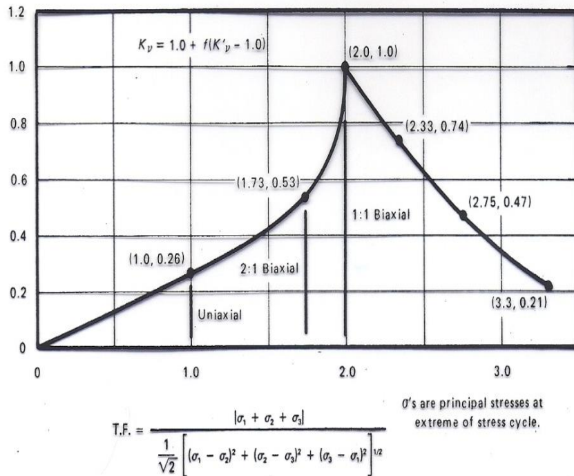
FIG. T-1432-2 INELASTIC MULTIAXIAL ADJUSTMENTS
