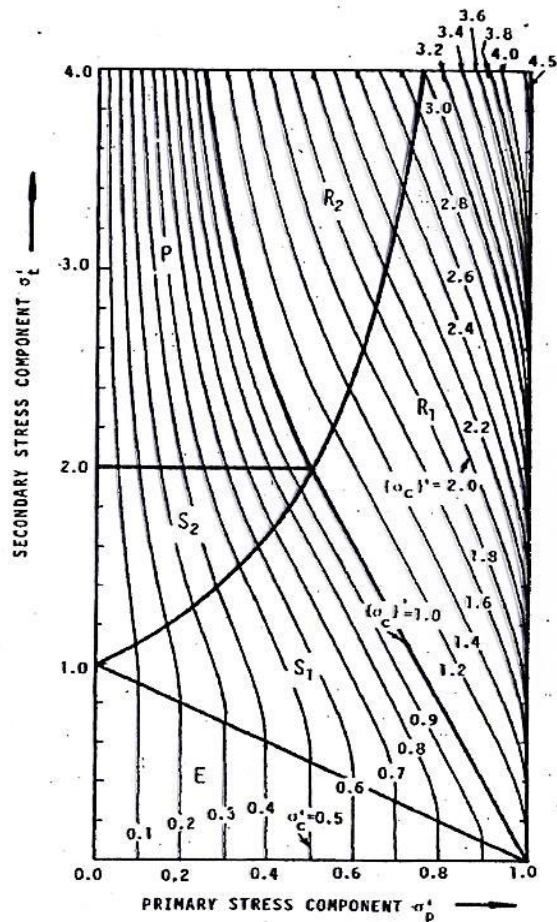
FIGURE 9 GENERALIZED CORE STRESS GRAPH
