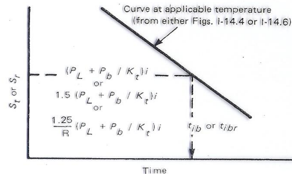
FIG. NH-3224-2 USE-FRACTIONS FOR MEMBRANE PLUS BENDING STRESS
