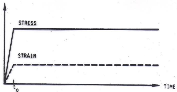
Fig. 1(a) HISTORIES FROM A LOADING AT LOW TEMPERATURE
