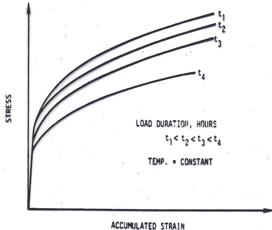
Fig. 5 ISOCHRONOUS STRESS-STRAIN CURVES FROM CREEP TESTS AT CONSTANT TEMPERATURE
