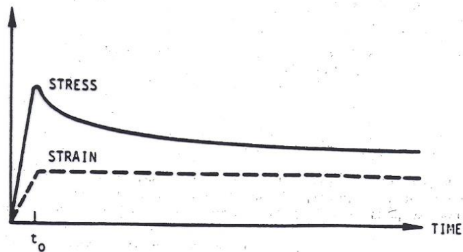
Fig. 1(c) HISTORIES FROM A STRAIN-CONTROLLED LOADING AT ELEVATED TEMPERATURE
