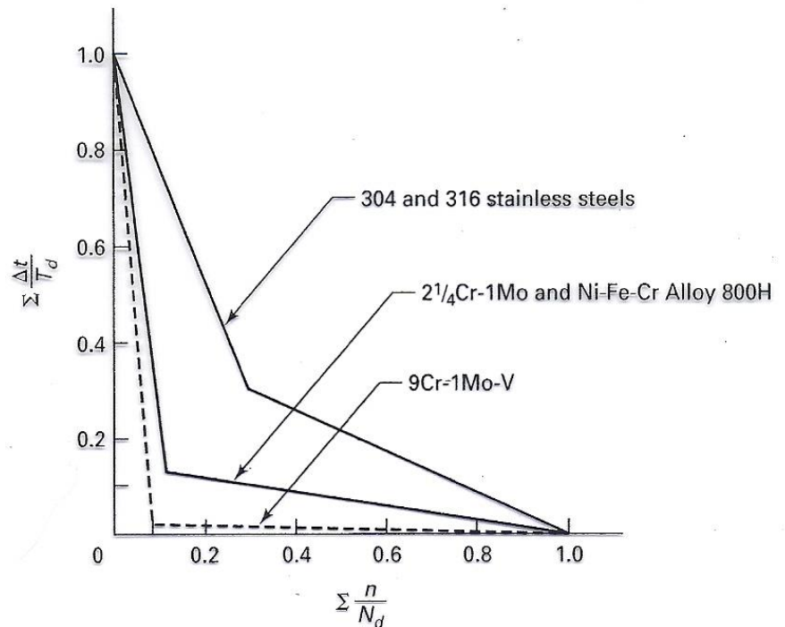
FIG. T-1420-2 CREEP-FATIGUE DAMAGE ENVELOPE
