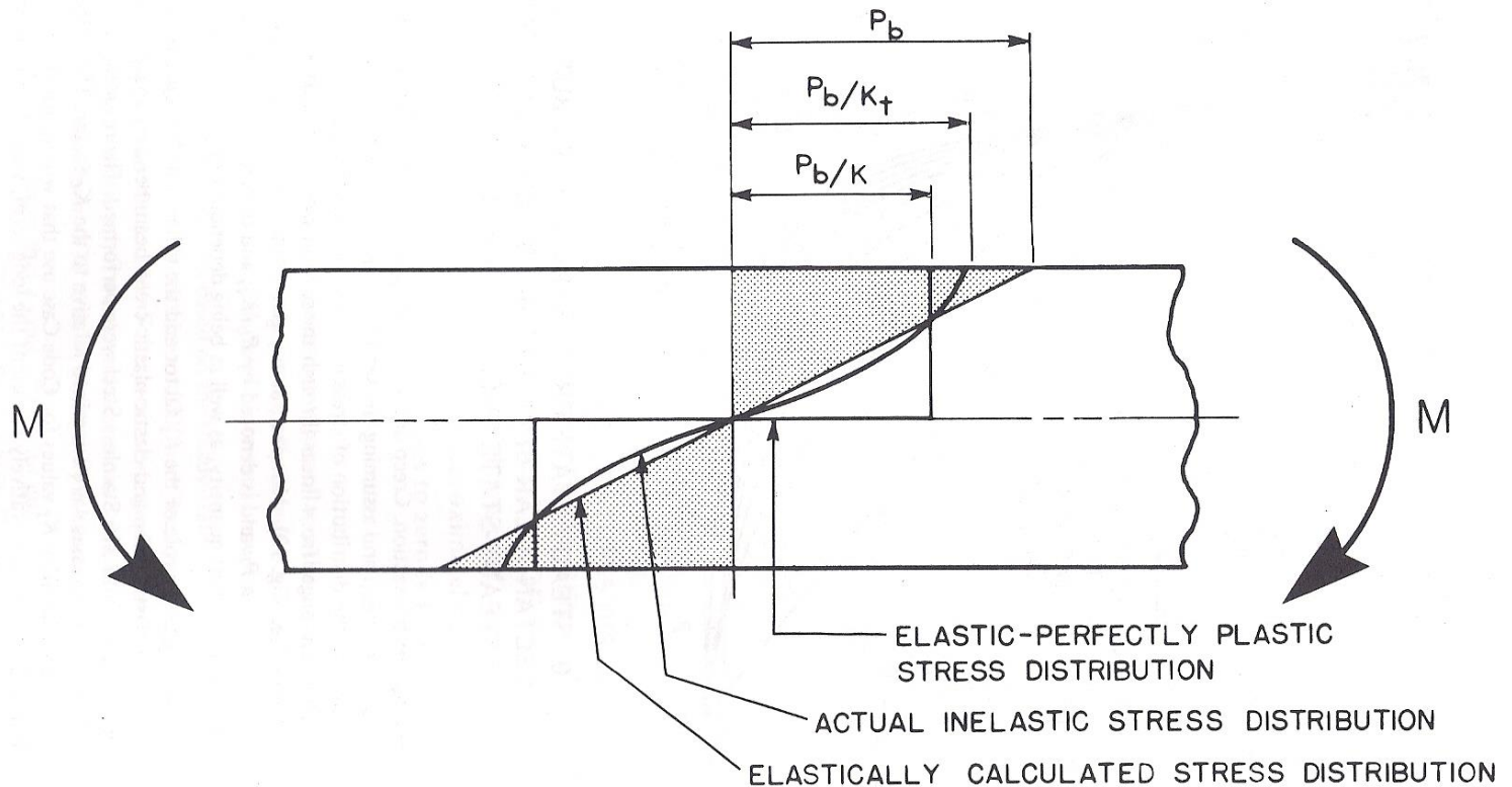
Fig. 9 ELASTICALLY CALCULATED PRIMARY BENDING STRESS DISTRIBUTION COMPARED TO ACTUAL TIME-DEPENDENT INELASTIC STRESS DISTRIBUTION
