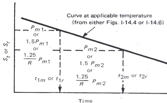
FIG. NH-3224-1 USE-FRACTIONS FOR MEMBRANE STRESS
