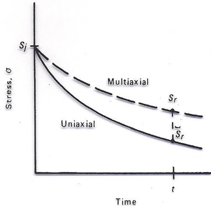
(b) Multiaxial Relaxation, S_r , Calculated from Uniaxial Relaxation, \bar{S}_r ,
