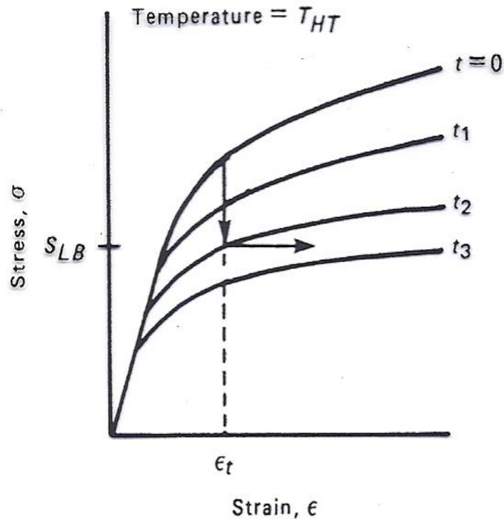
(a) Stress Relaxation from Isochronous Stress-Strain Curves
