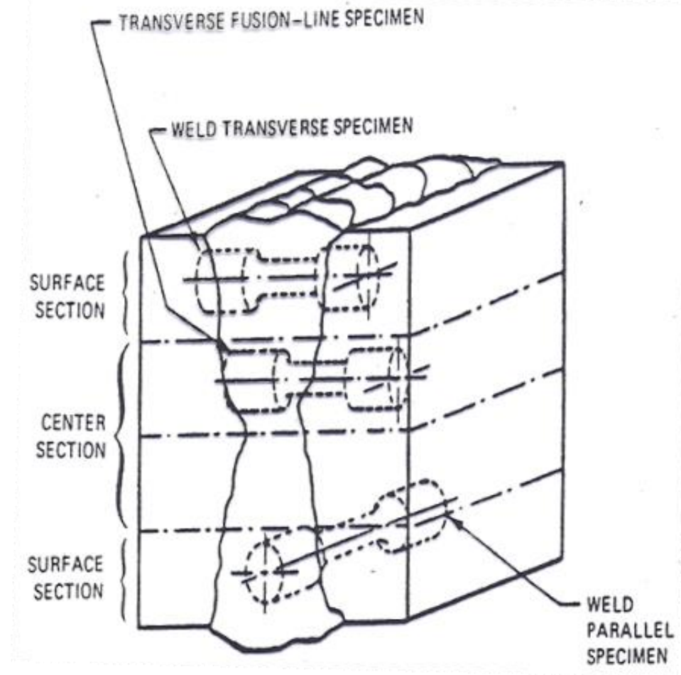
Location/orientation of three types of uniaxial Fatigue and creep-fatigue specimen taken from weldments
