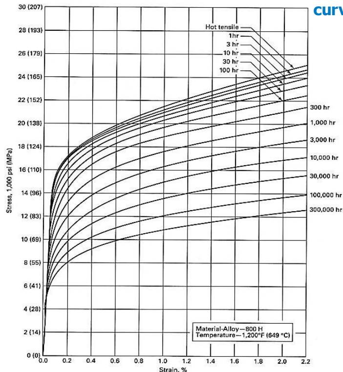
Figure T-1800-C-8 Average Isochronous Stress-Strain Curves
