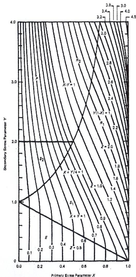
FIG. T-1332-1 EFFECTIVE CREEP STRESS PARAMETER Z FOR SIMPLIFIED INELASTIC ANALYSIS USING TEST NOS. B-1 AND B-3 [For Use Only When the Restrictions of T-1331(a) for Test No. B-1 Are Met]
