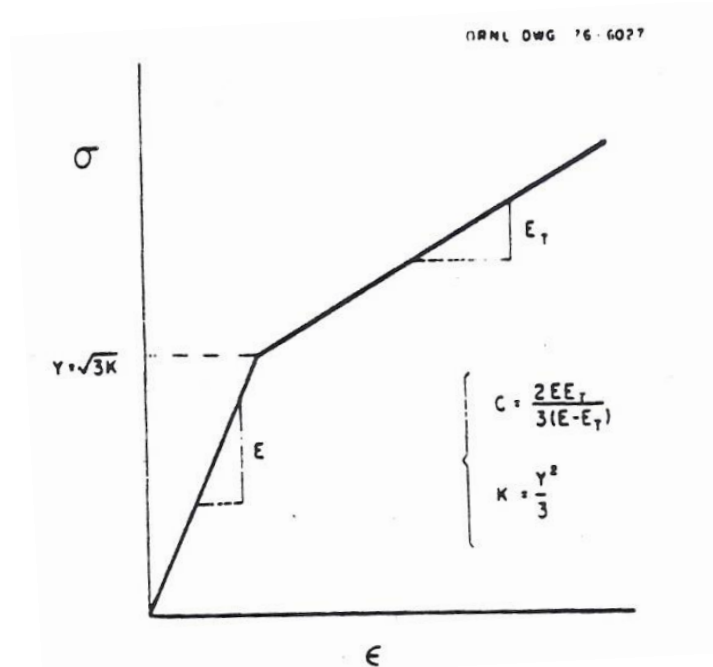
Bilinear idealization of material stress-strain curve giving definition of X and C
