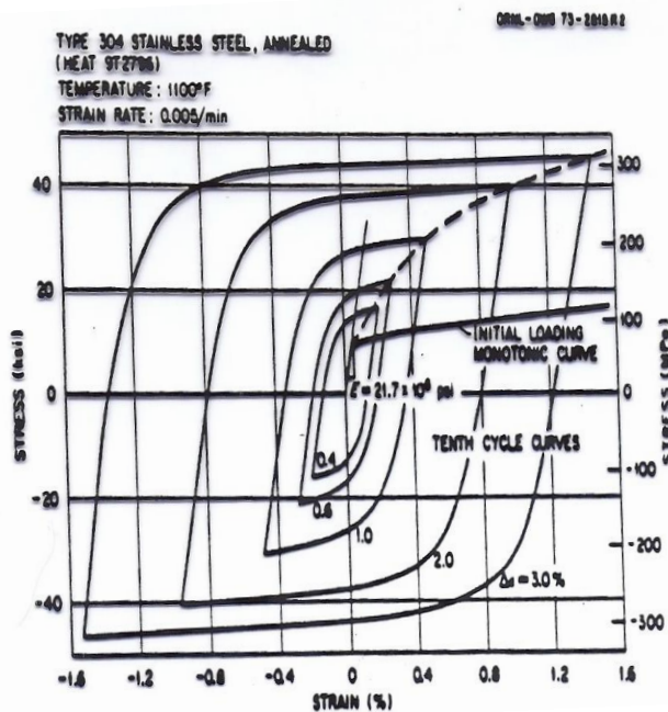
Monotonic Loading Stress-Strain Curve and Tenth-Cycle Stress-Strain Curves for Different Total-Stress Ranges. Annealed Type 304 Stainless Steel at 593°C (1100°F)
