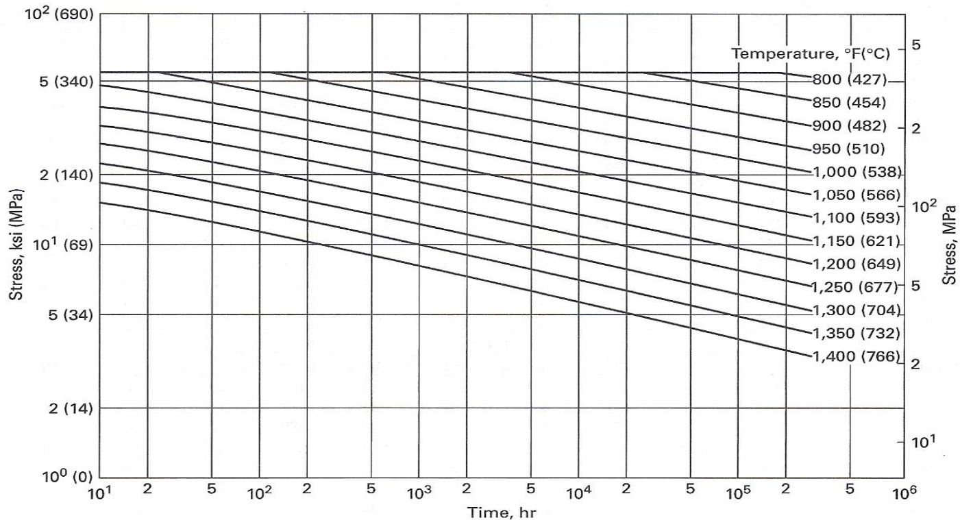
Minimum Stress-to-Rupture — Ni-Fe-Cr (Alloy 800H)
