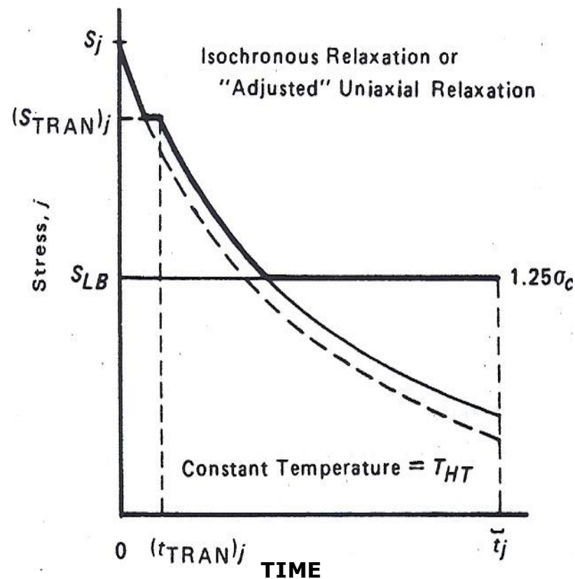
Load Controlled Transient Effects
