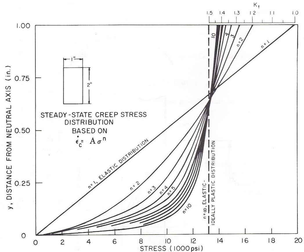
Fig. 10 STEADY-STATE CREEP STRESS DISTRIBUTION ACROSS A RECTANGULAR BEAM IN PURE BENDING AND HAVING A STEADY-STATE CREEP LAW OF THE FORM, \dot{\epsilon}_c = A\sigma^n
