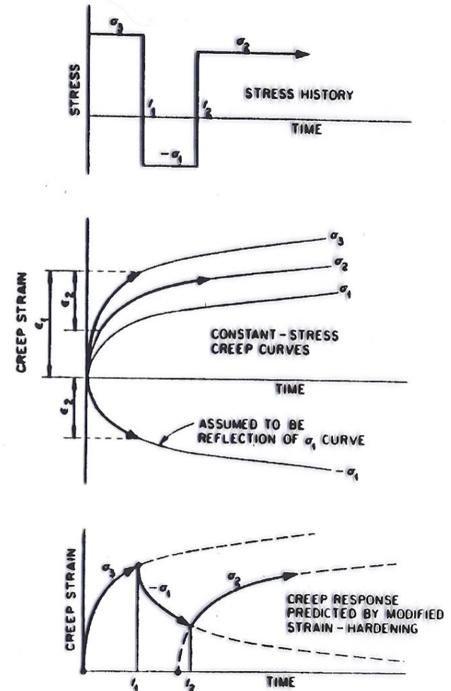
Fig. 2 Axial creep strain response predicted by auxiliary procedures for reversed uniaxial creep loads.
