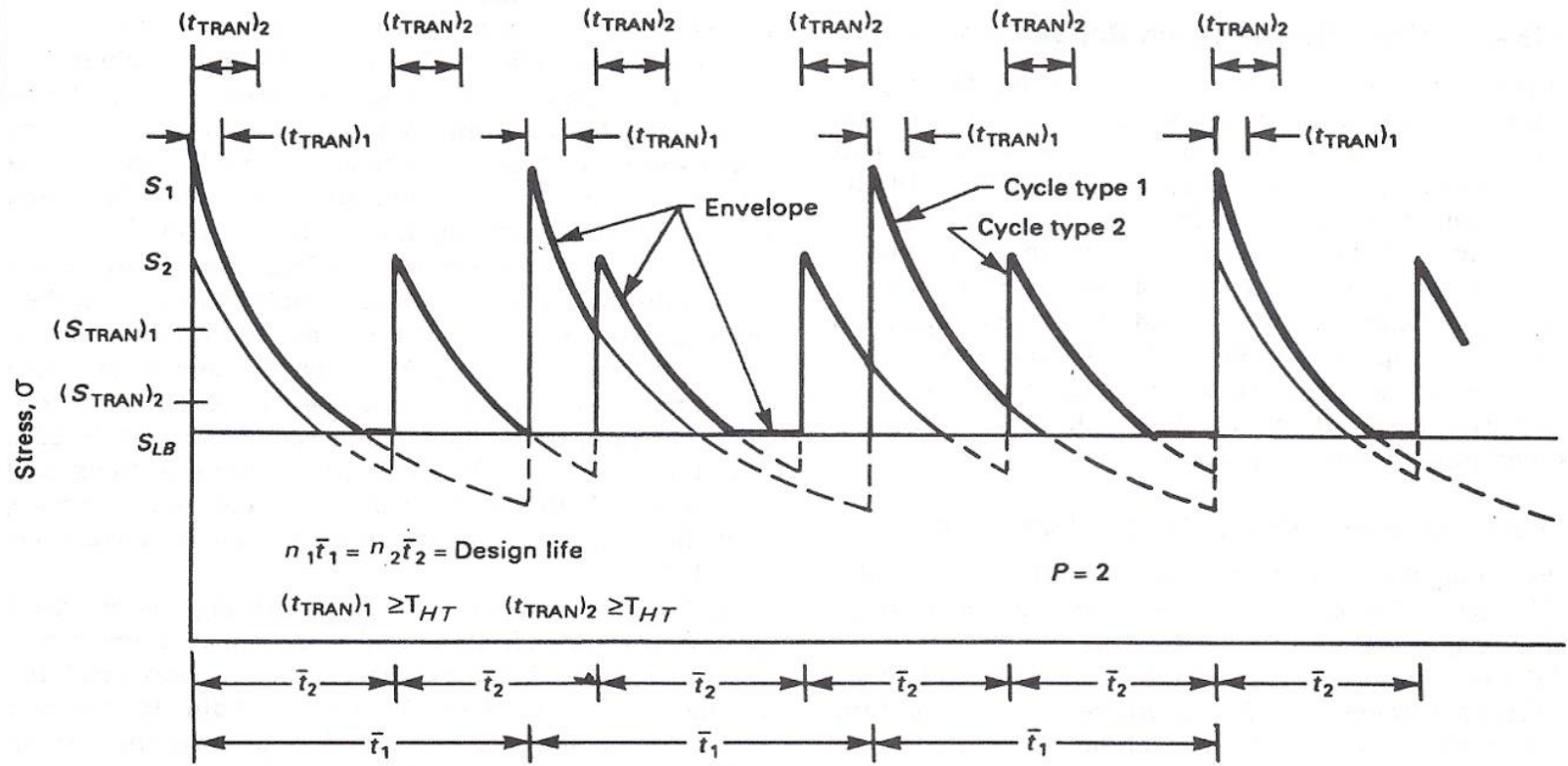
Envelope Stress-Time History for Creep Damage Assessment
