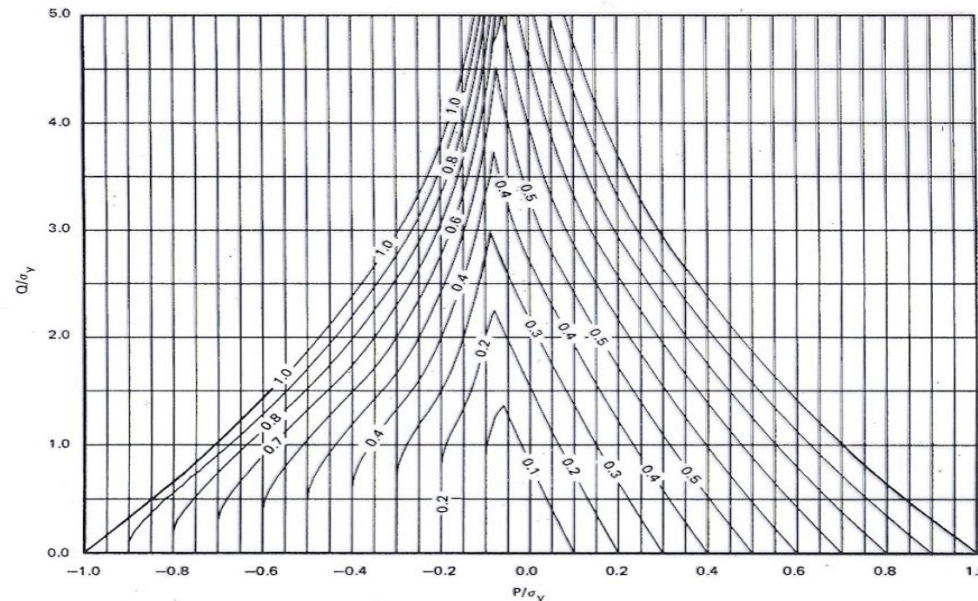
Fig. 4. Design chart of elastic core stress contours obtained from equation |\sigma_c| = f(Q) |\sigma_c|_{\text{closed form}} (P,Q) and correlated in terms of dimensionless secondary or Q stress and primary stress.
