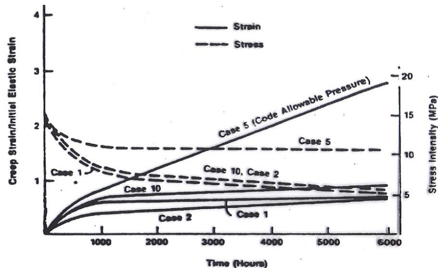
FIG. 12.36 STRESS RELAXATION AND STRAIN ACCUMULATION FOR PRESSURE DISCONTINUITY (CASE 5), THERMAL DISCONTINUITY (CASE 10), AND SECONDARY STRESS (CASES 1, 2)
