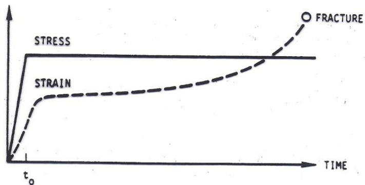
Fig. 1(b) HISTORIES FROM A LOAD-CONTROLLED LOADING AT ELEVATED TEMPERATURE
