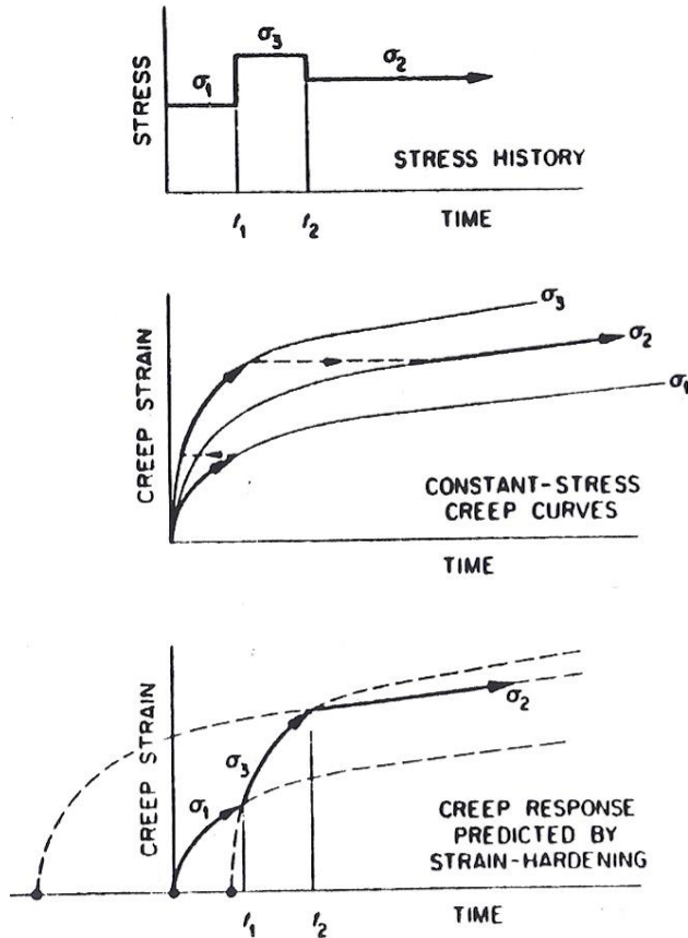
Fig. 1 Axial creep strains predicted by strain-hardening analysis (based on total creep strains) for variable uniaxial loads in the absence of stress reversals.
