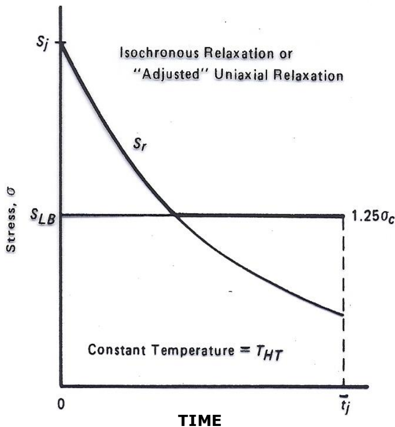
Fig. T-1433-2 Stress-Relaxation Limits for Creep Damage
