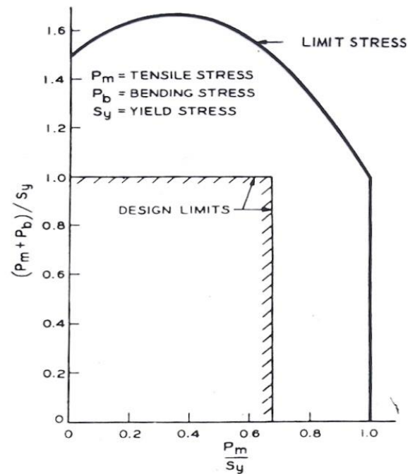
FIGURE 2. LIMIT STRESS FOR COMBINED TENSION AND BENDING (RECTANGULAR SECTION)
