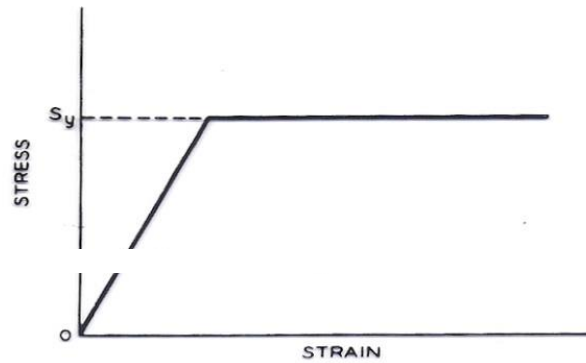
FIGURE 1. IDEALIZED STRESS - STRAIN RELATIONSHIP
