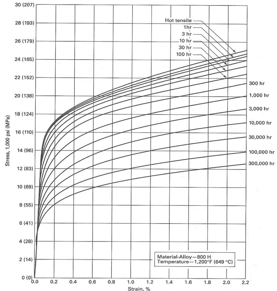
Average Isochronous Stress-Strain Curves
