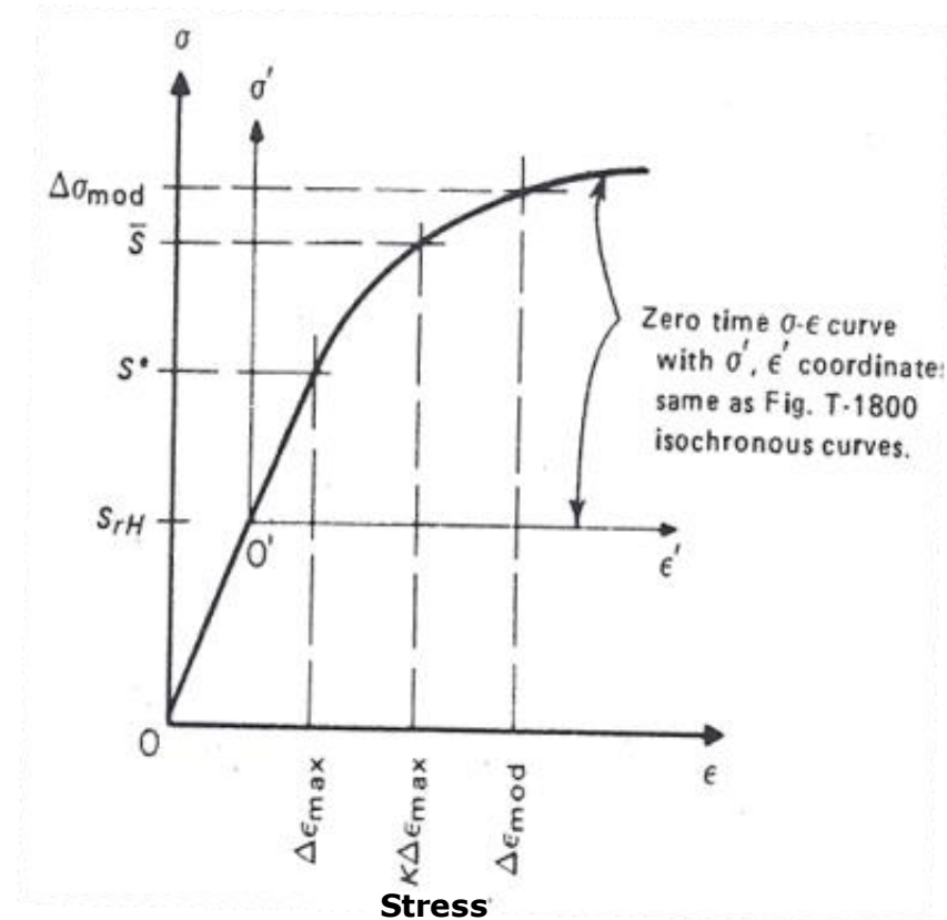
Fig. T-1432-1 Stress-Strain Relationship
