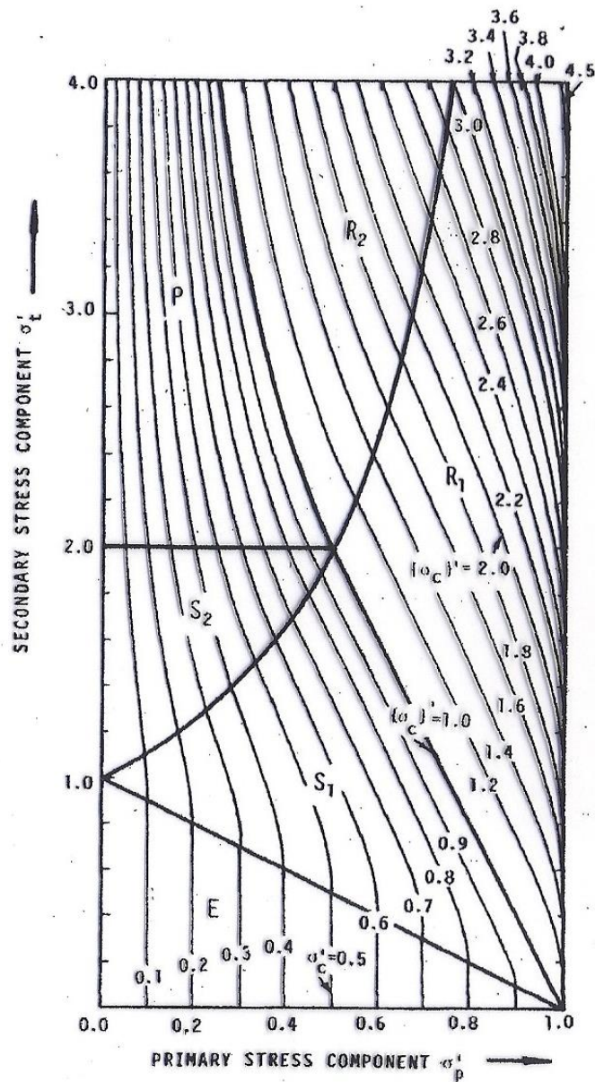
FIGURE 9 GENERALIZED CORE STRESS GRAPH
