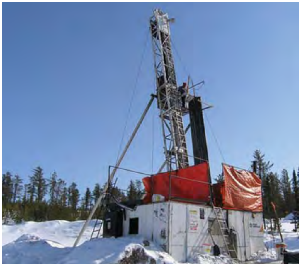
Winter drilling at Millenium Mine.
