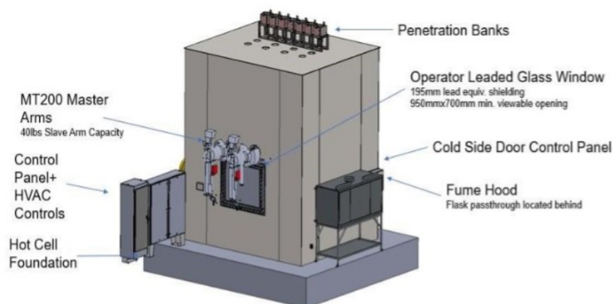
Figure 2. Overview of the proposed hot cell design [4].
