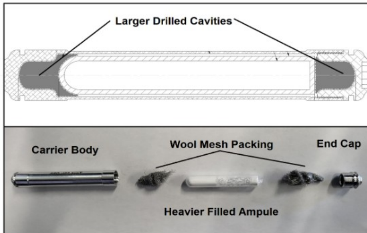
Figure 3. Lu-177 target assembly overview [4].
