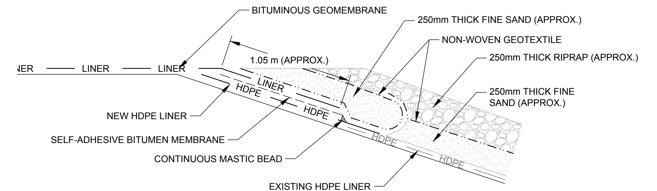
SCALE 1:20 5 DETAIL -
