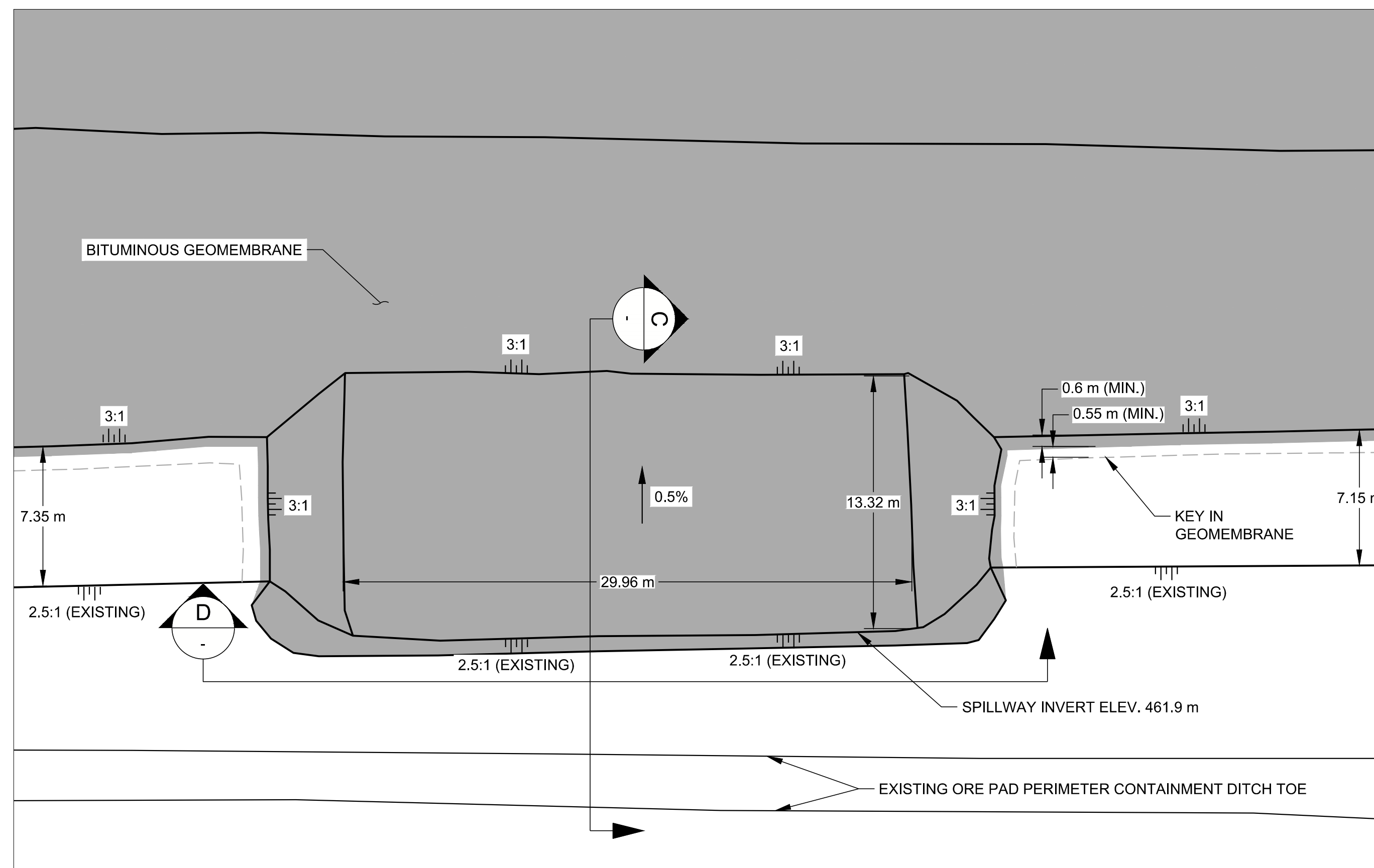
SCALE 1:200 1 LINED OVERFLOW SPILLWAY DETAIL 403
