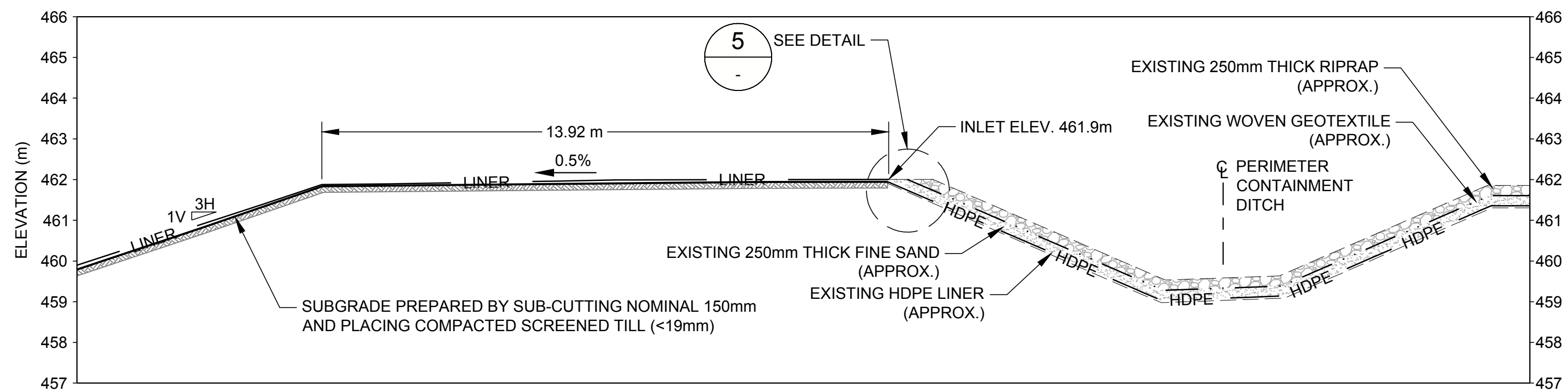
SCALE 1:100 C CROSS SECTION C -
