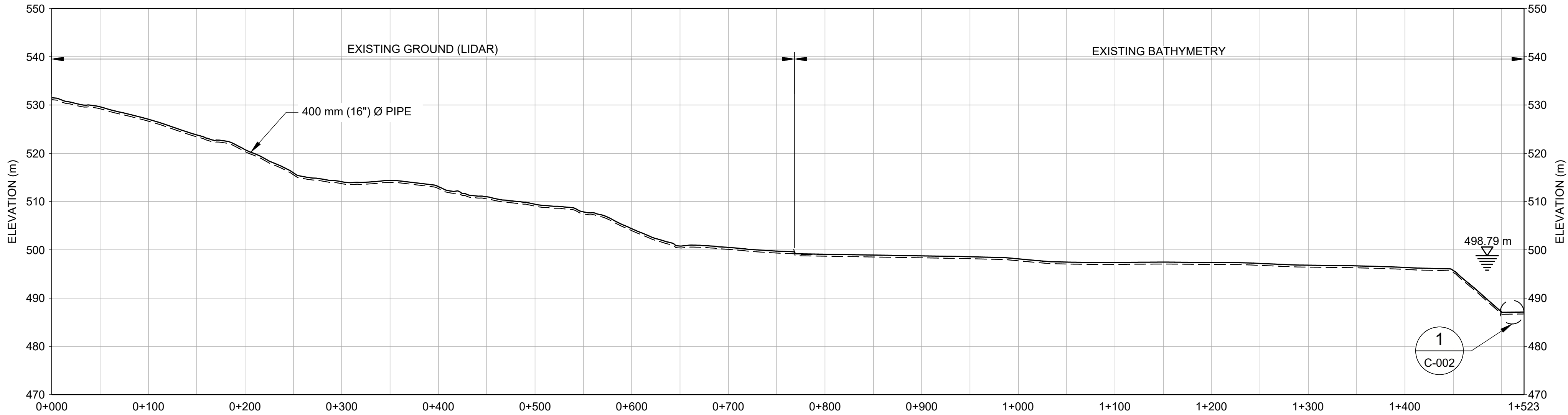
PROFILE - PROPOSED DIFFUSER PIPELINE SCALE 1:3,000 VERT. SCALE 1:600
