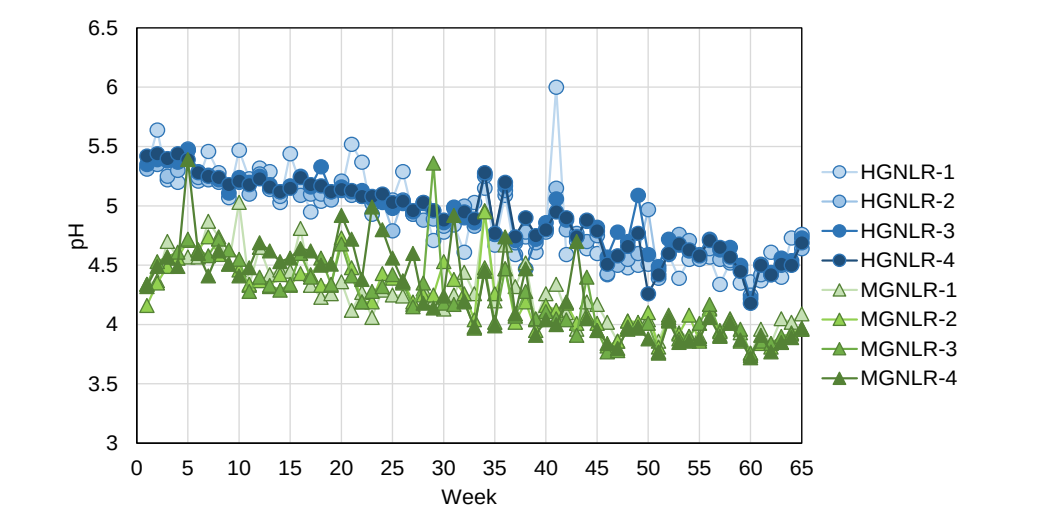
Figure F2-29: HCT Leachate pH vs Time
