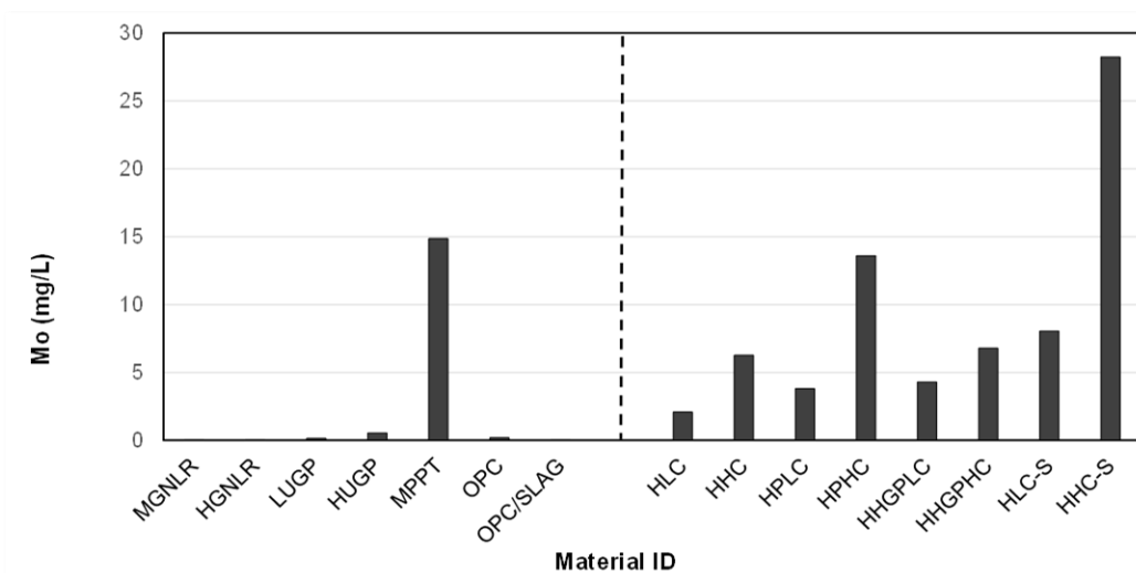
Figure D2-30: SFE Molybdenum Concentration vs Material Type
