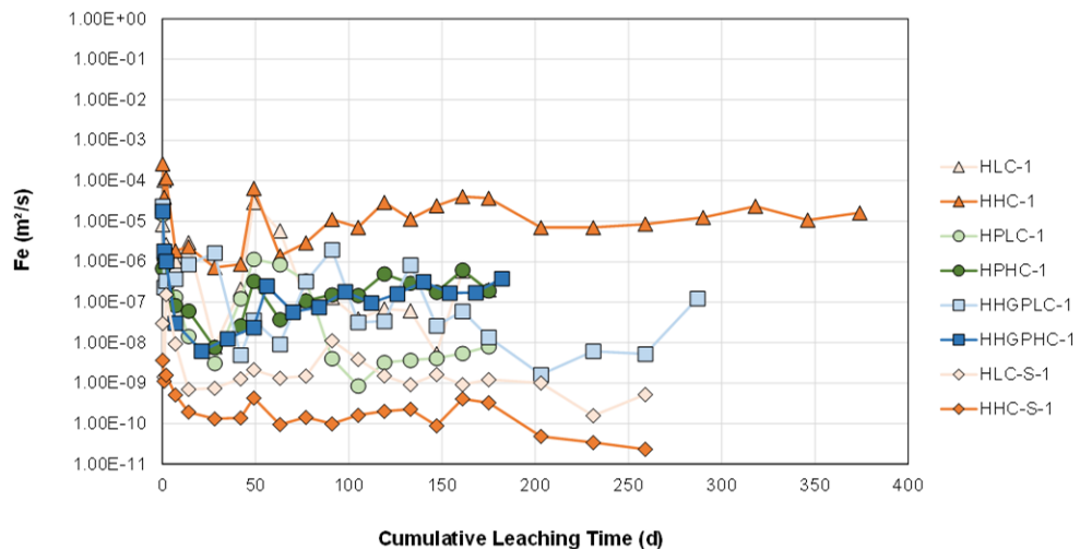
Figure F4-18: Iron Diffusivity vs Cumulative Leaching Time
