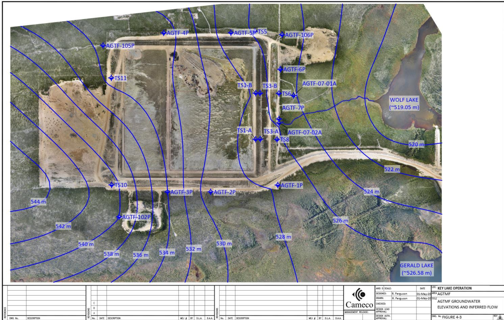
Figure 3.4: Groundwater flow directions at the AGTMF [63]
