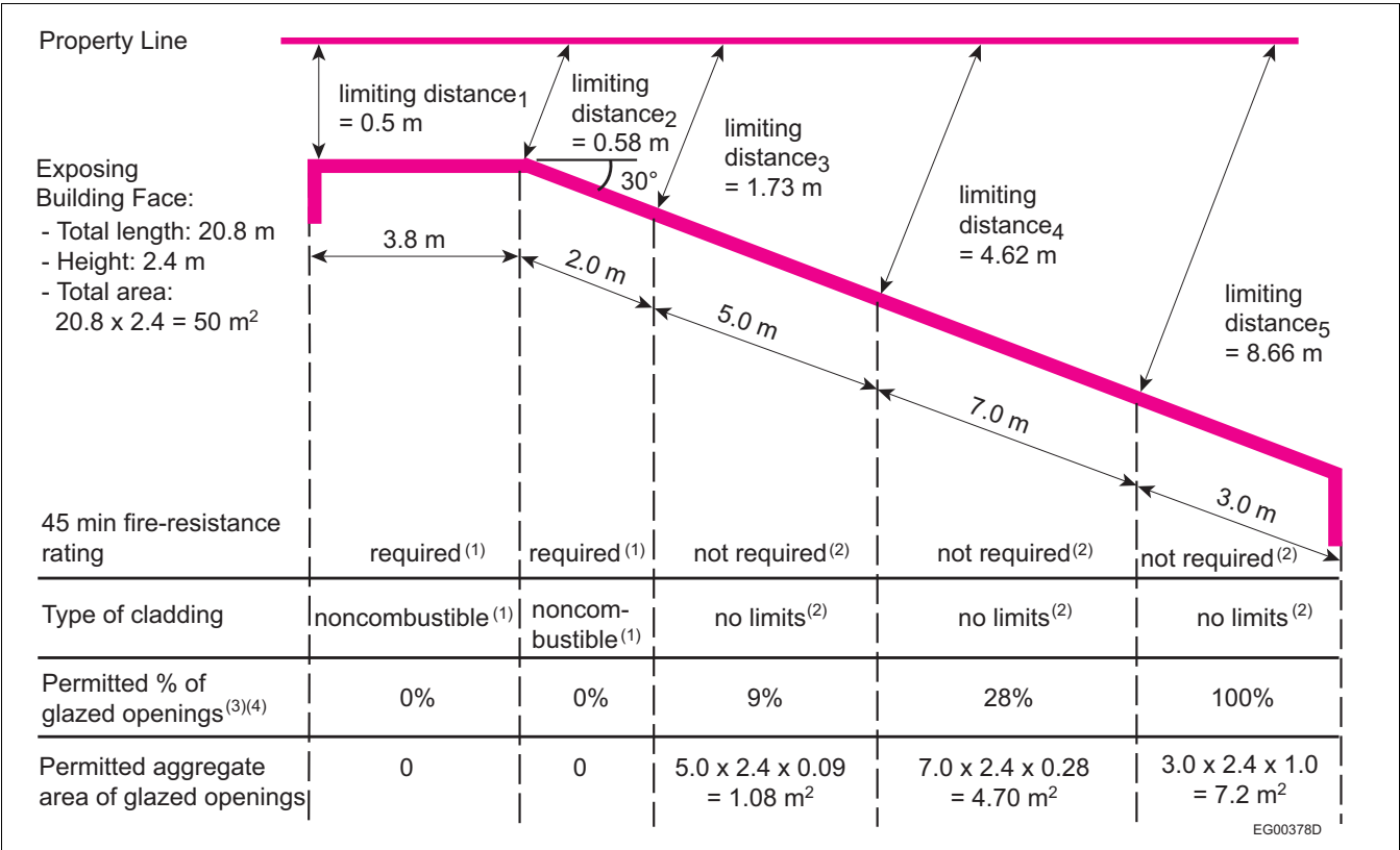
Figure A-9.10.15.4.(2)-B Example of determination of criteria for the exposing building face of a skewed wall of a house with some arbitrary division of the wall (plan view)
