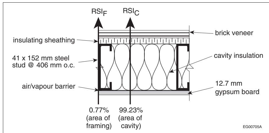
Figure 2-1 RSI_{eff} calculation parameters for a 41 × 152 mm steel-frame wall assembly
