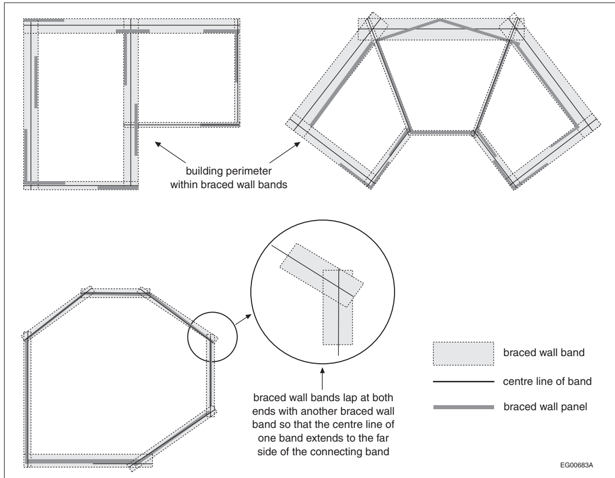
Figure A-9.23.13.4-B
