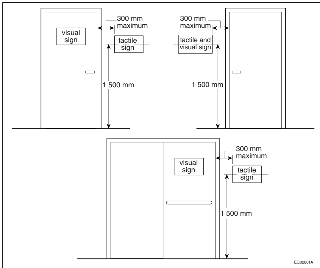
Figure A-3.8.3.9.(1) and (2) Positioning of visual and tactile information signs on and near doors
