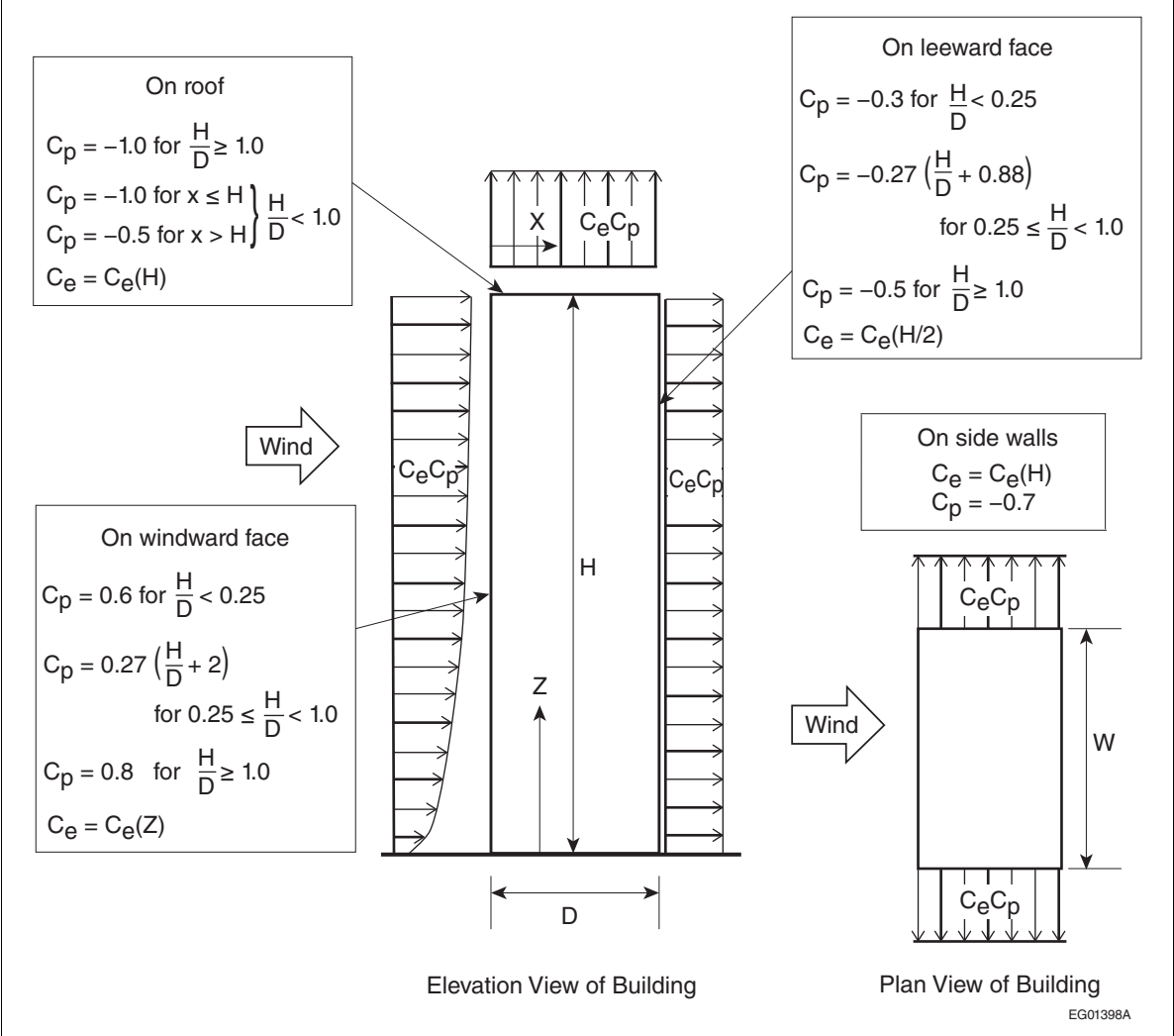
Figure A-4.1.7.5.(2) and (3) Values of C_p for main structural system on rectangular buildings
