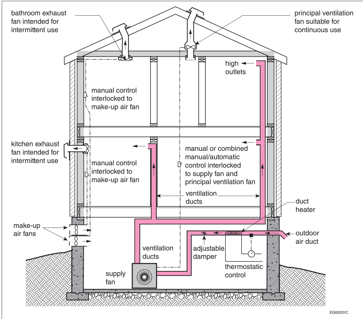
Figure A-9.32.3.3.-C Possible configuration of a mechanical ventilation system not coupled with a forced air heating system Note to Figure A-9.32.3.3.-C:
