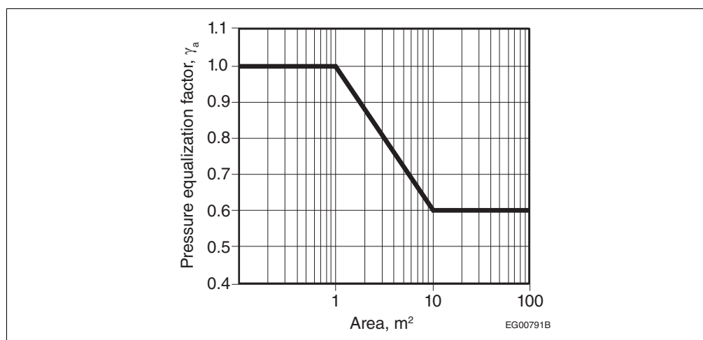
Figure 4.1.7.13.-A Pressure equalization factor, \gamma_a , for solar panels or arrays mounted on roofs of buildings of any height Forming Part of Clause 4.1.7.13.(3)(b)
