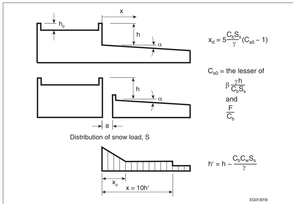
Figure 4.1.6.5.-A Snow load factors for lower level roofs
