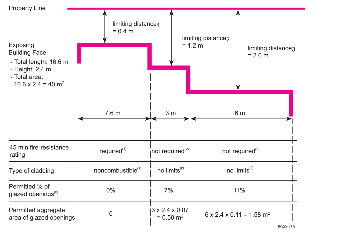
Figure A-9.10.15.4.(2)-A Example of determination of criteria for the exposing building face of a staggered wall of a house (plan view)
