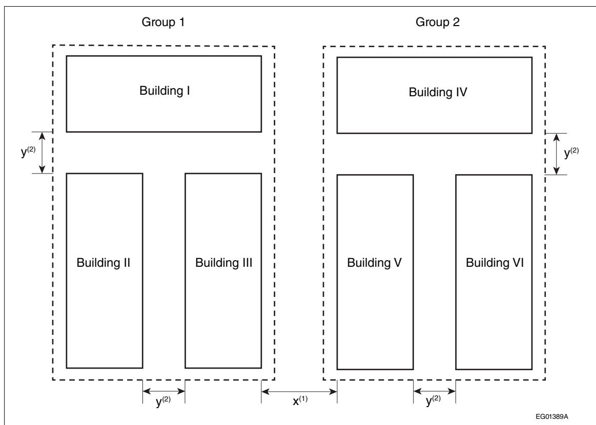
Figure A-3.9.2.2.
