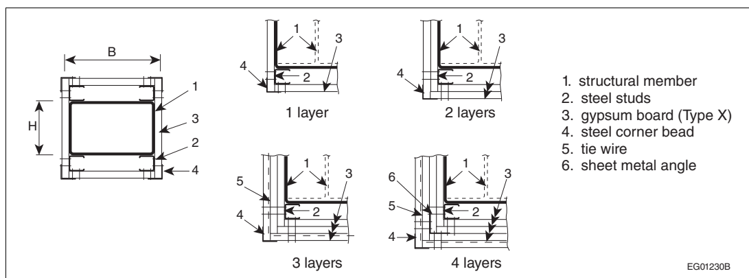
Figure D-2.6.4.-B
