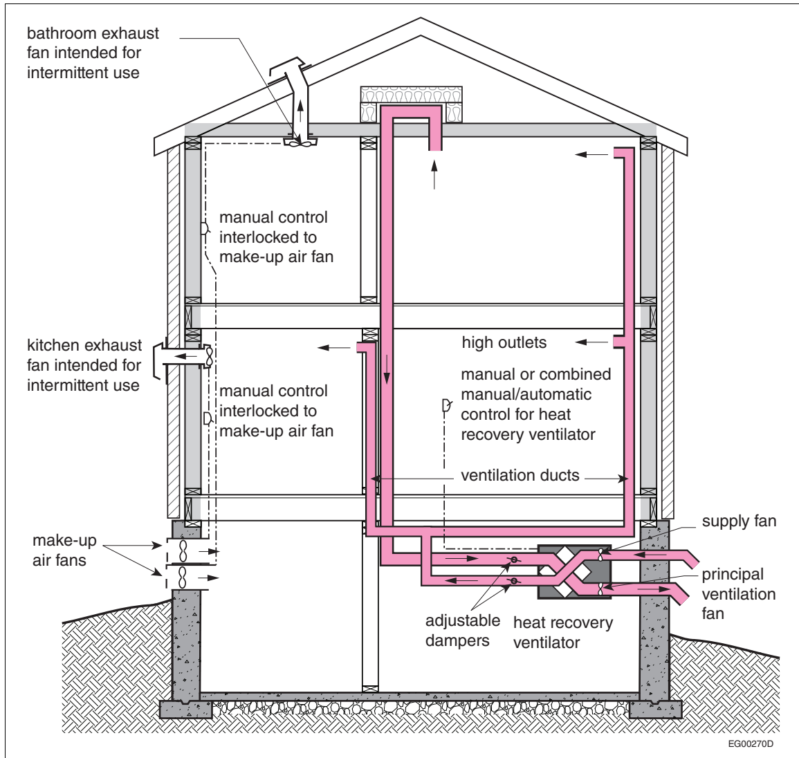
Figure A-9.32.3.3.-D
